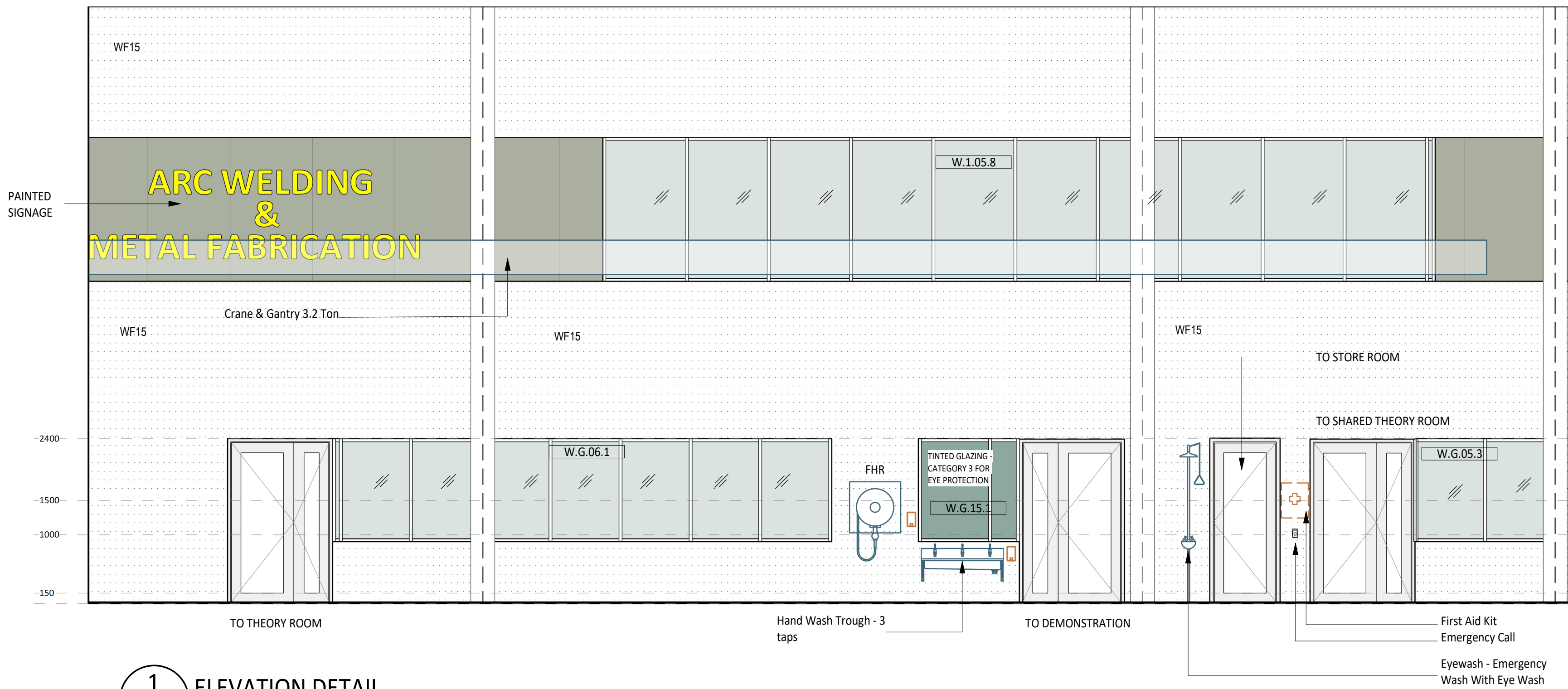
1 60-011 ELEVATION DETAIL 1 : 50
