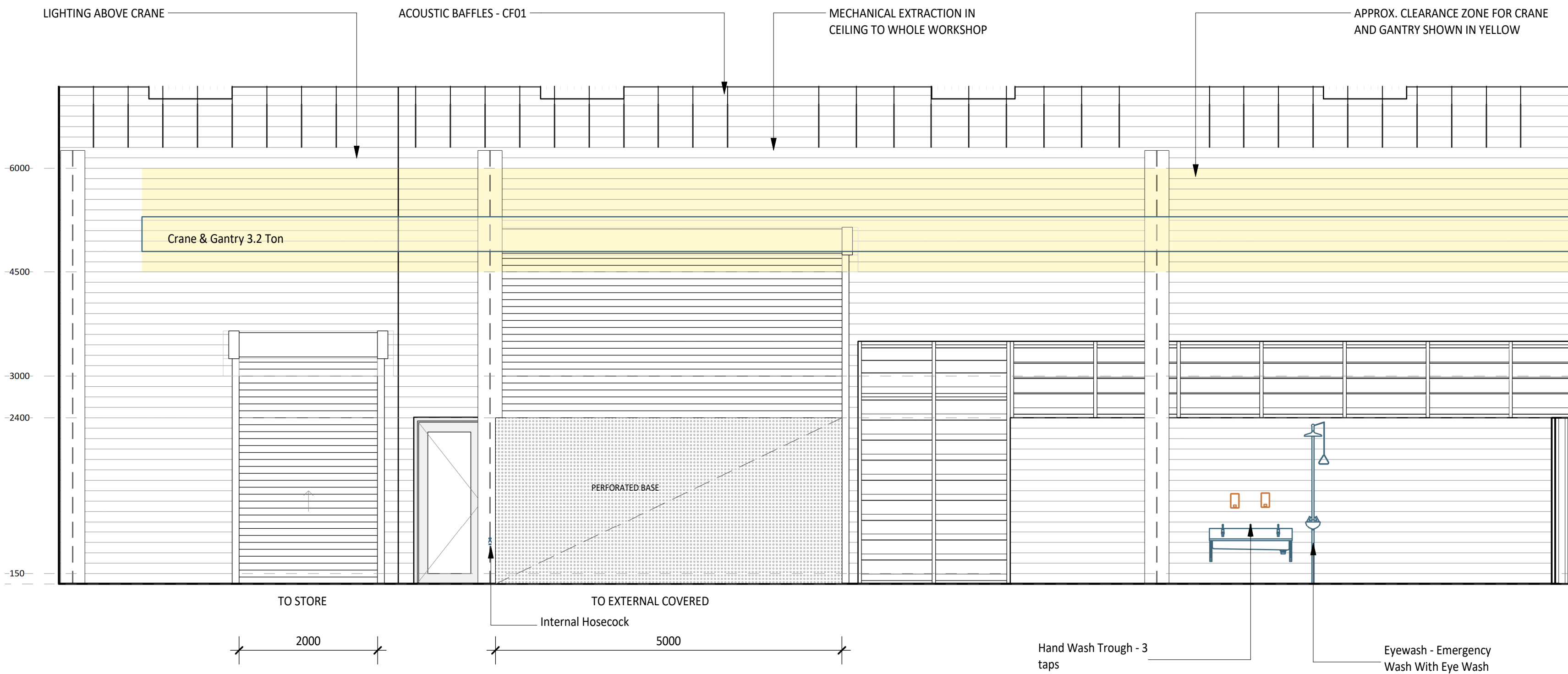
2 60-011 ELEVATION DETAIL 1 : 50
